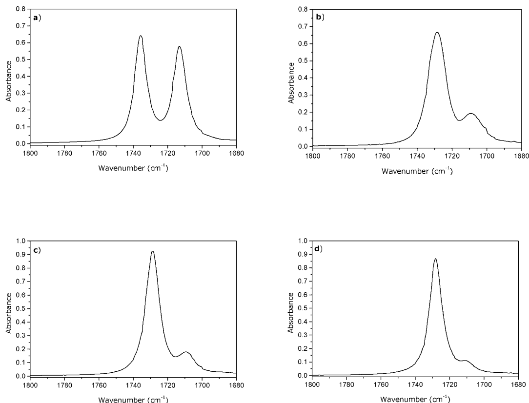
Figure 3. The carbonyl absorption band in the IR spectrum of FDMB in (a) \text{CCl}_4 , (b) \text{CHCl}_3 , (c) \text{CH}_2\text{Cl}_2 and (d) \text{CH}_3\text{CN}
