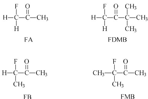
Figure 4. Structural formulae of fluoroketones
