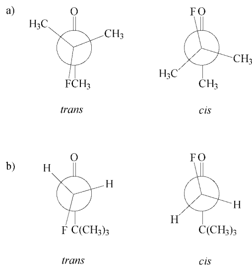
Figure 1. (a) Rotamers trans and cis for FMB; (b) rotamers trans and cis for FDMB
