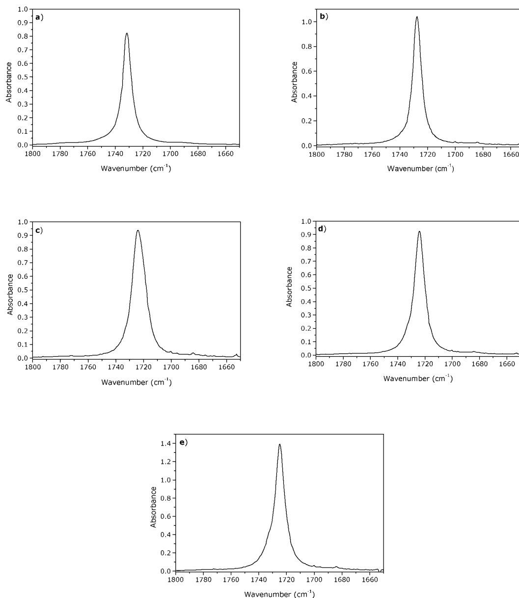
Figure 2. The carbonyl absorption band in the IR spectrum of FMB in (a) hexane, (b) \text{CCl}_4 , (c) \text{CHCl}_3 , (d) \text{CH}_2\text{Cl}_2 and (e) \text{CH}_3\text{CN}
